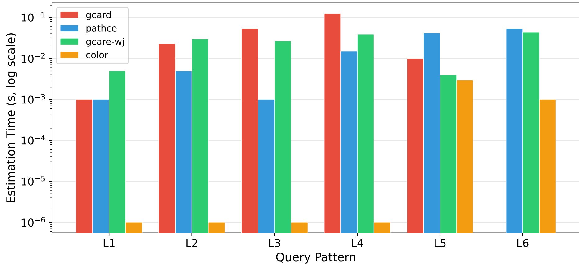
Estimation Time (Without Predicates, SF1)
