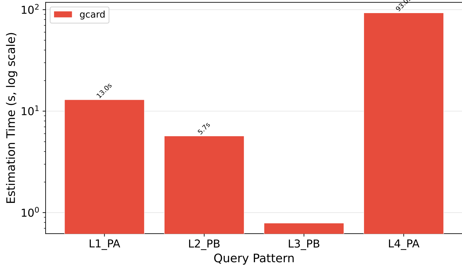
Estimation Time (With Predicates, SF1)
