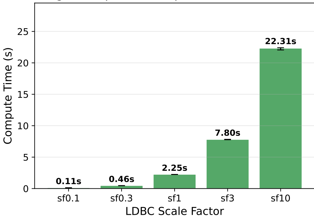
Degree Sequence Compute Time (24 threads)
