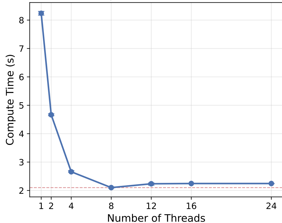
Compute Time vs Threads
