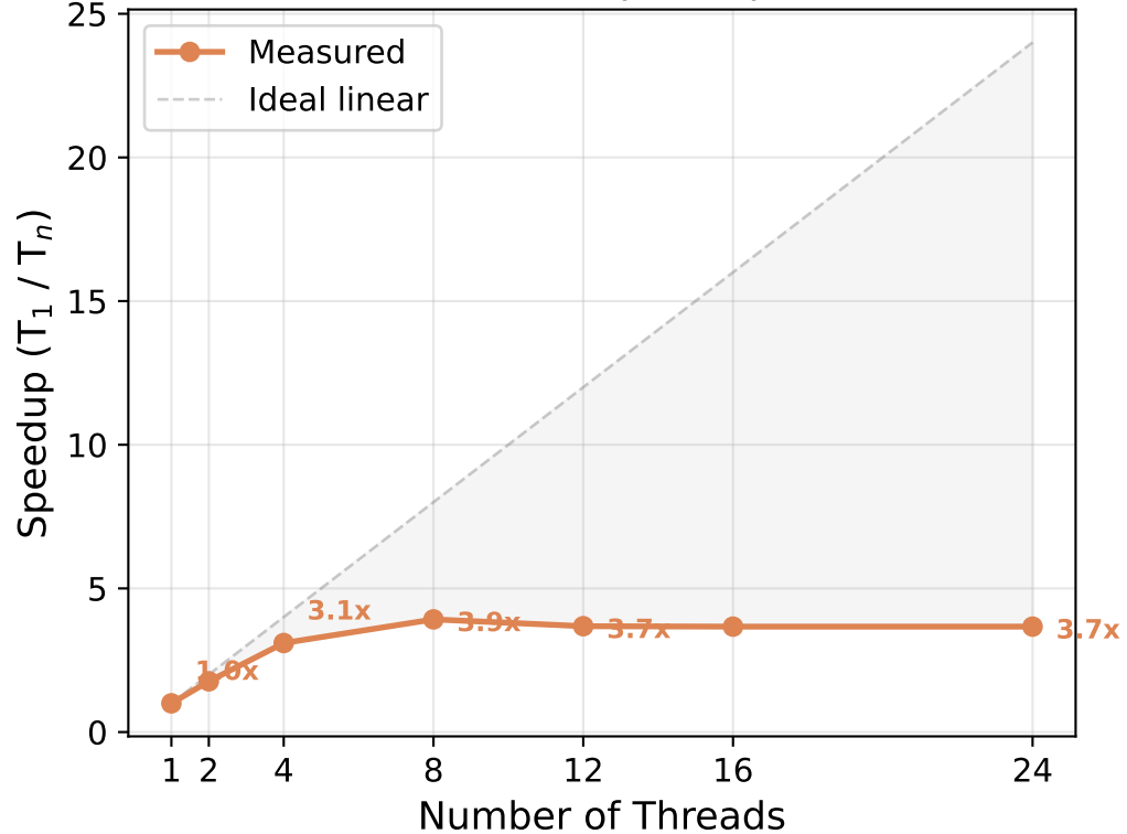
Parallel Speedup
