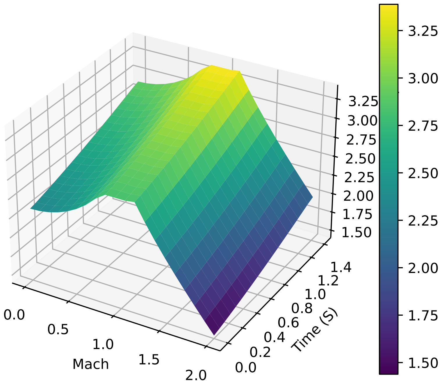
Stability Margin (C) x Mach x Time (S)
