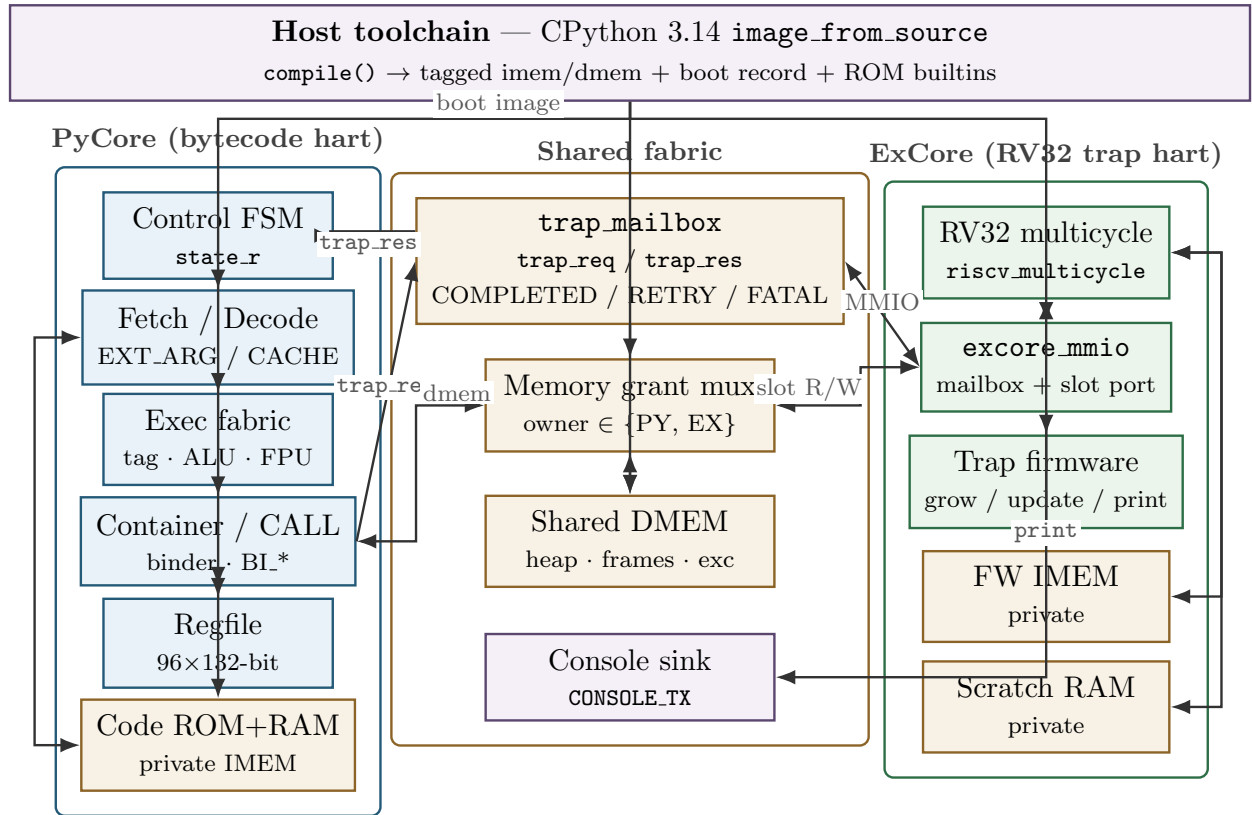
Figure 1: System block diagram of pycore_excore_system . PyCore and ExCore keep private instruction memories; the shared DMEM is reached only through the exclusive grant mux. Recoverable traps cross trap_mailbox into ExCore MMIO/firmware; CONSOLE.TX is the print sink.
