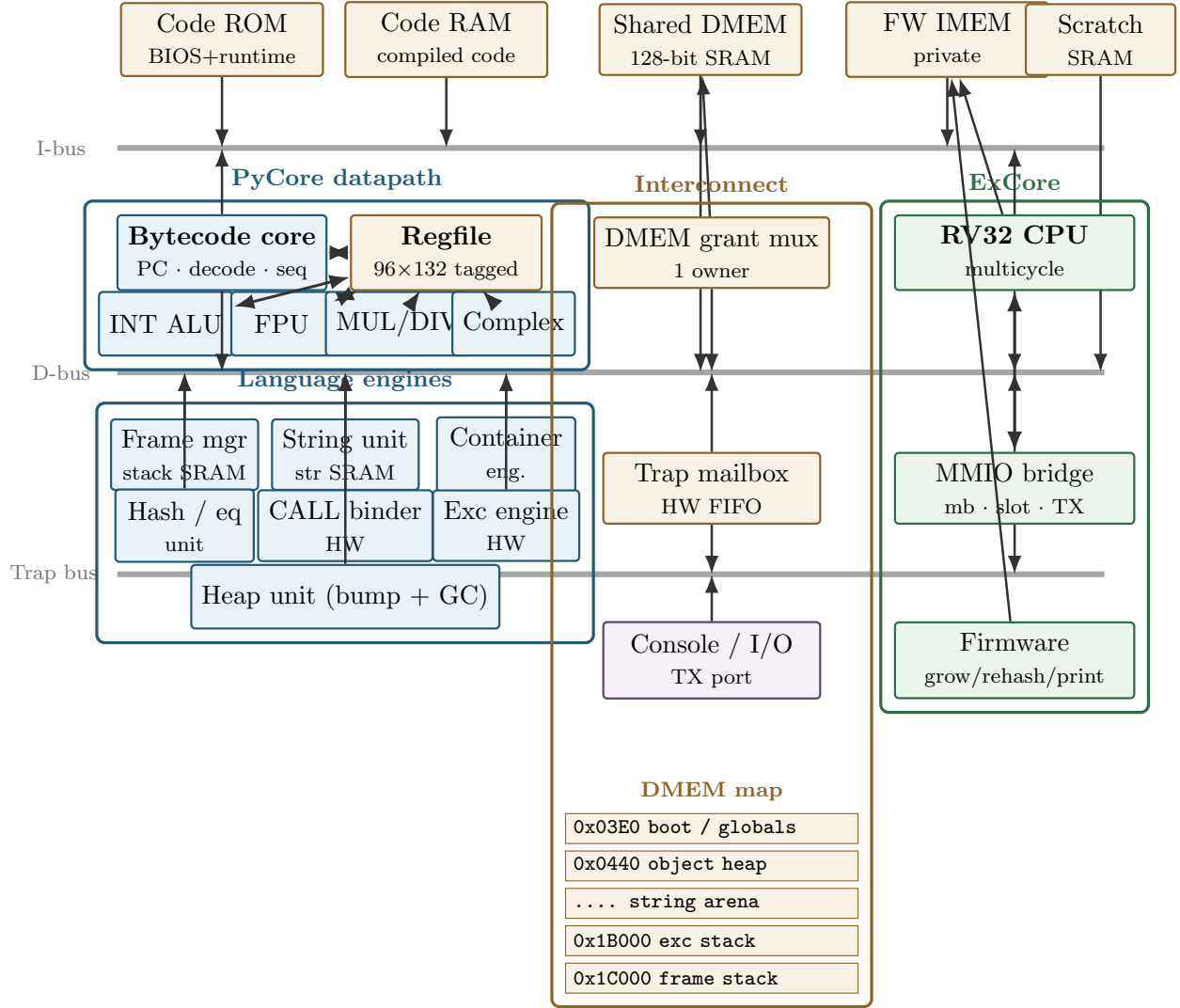
Figure 1: Physical SoC view: memories on the I-bus and D-bus, PyCore datapath and language engines as peer hardware blocks, ExCore as an RV32 CPU behind an MMIO bridge, and a trap mailbox on a dedicated bus. The DMEM map lists the principal shared address regions. No control-pipeline stages are shown.
