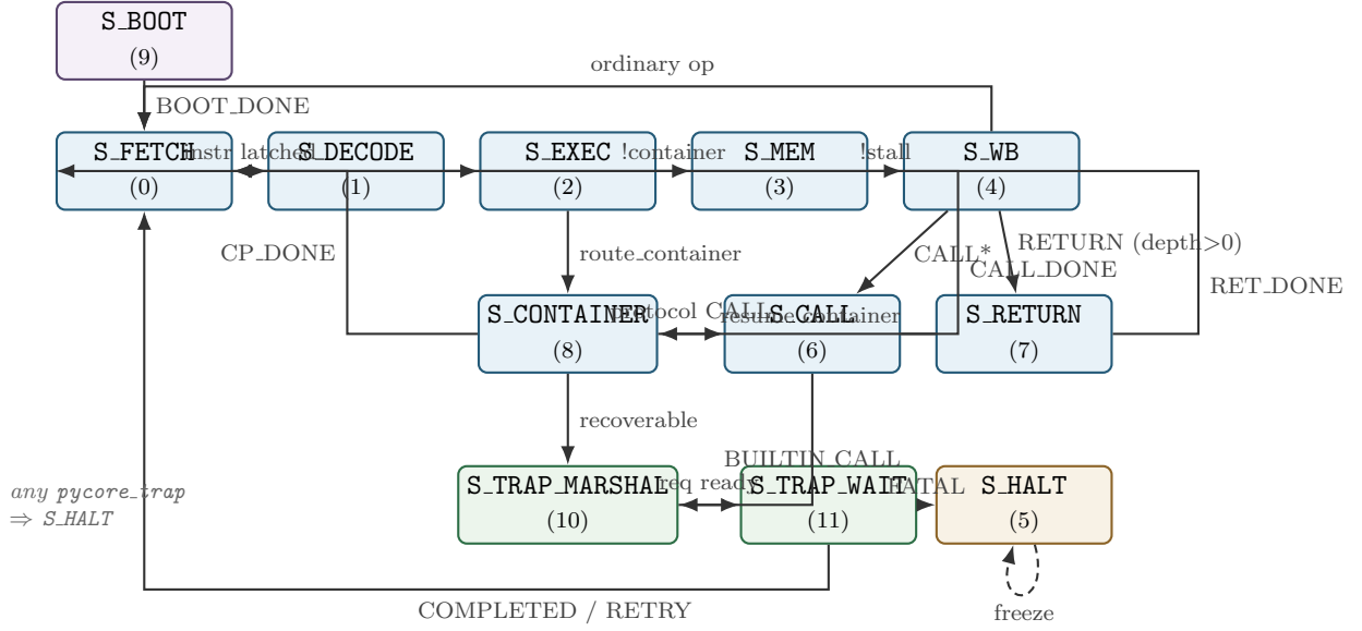
Figure 2: PyCore top-level control FSM ( state_r ). The five-stage strip is the typed fast path. S_CONTAINER and S_CALL / S_RETURN bypass or follow writeback for heap and frame work; recoverable traps exit through S_TRAP_MARSHAL / S_TRAP_WAIT to ExCore. Protocol iteration pauses S_CONTAINER , runs S_CALL , and resumes via S_RETURN .
