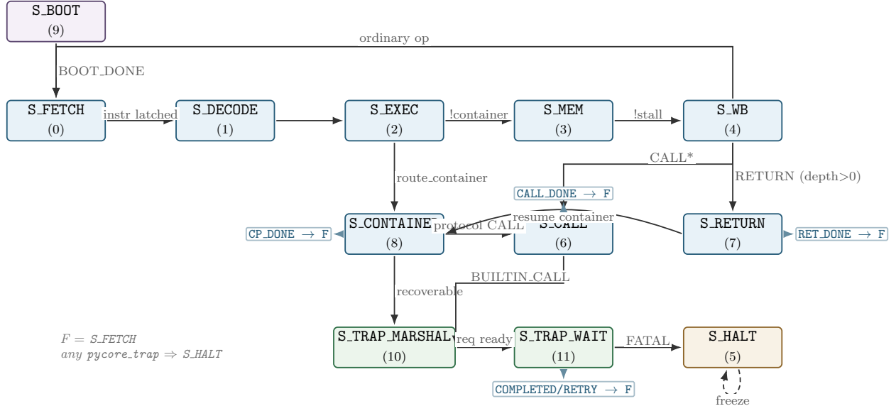
Figure 2: PyCore top-level control FSM ( state_r ). Solid arrows are local control transfers. Dashed exit tags mark returns to S_FETCH without wrap-around wires. The five-stage strip is the typed fast path; S_CONTAINER / S_CALL / S_RETURN handle heap and frames; recoverable traps exit through S_TRAP_MARSHAL / S_TRAP_WAIT .
