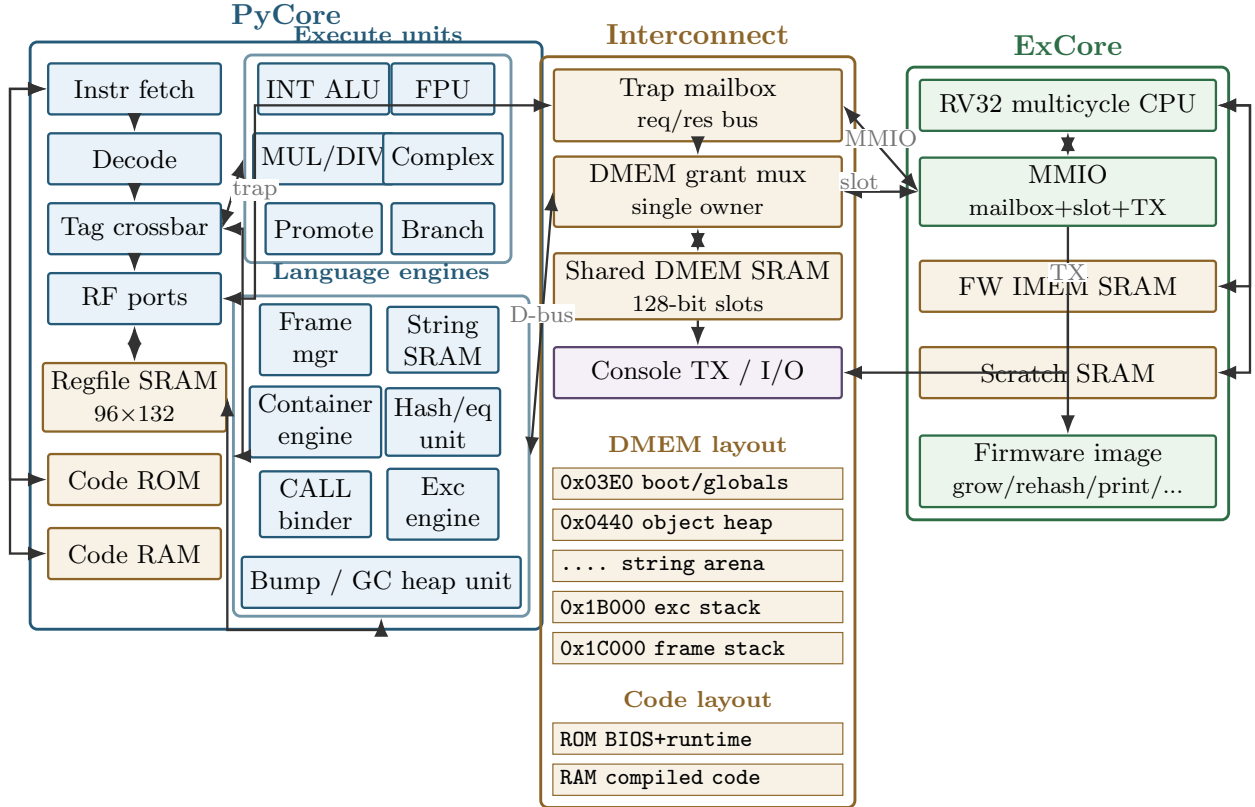
Figure 1: Physical hardware of the ideal machine: SRAMs, execute units, language engines, interconnect, and the RV32 helper core. PyCore owns a tagged regfile, private code ROM/RAM, typed ALUs, and engines for frames, strings, containers, hashing, calls, exceptions, and heap allocation. ExCore is an RV32 CPU with private IMEM/scratch and MMIO onto the trap mailbox, DMEM slot port, and console. Shared DMEM is single-owner through the grant mux; addresses show the memory map.
