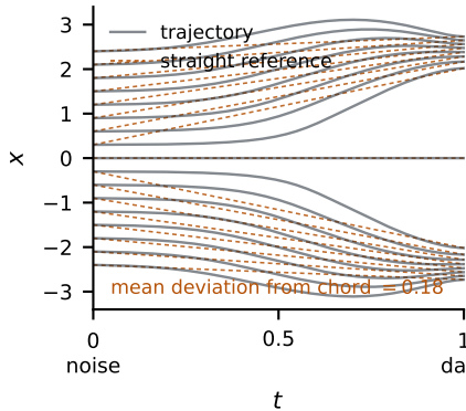
(a) diffusion probability flow
