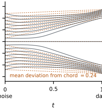
(b) rectified flow, independent coupling
