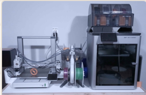
3D printers Bambu Lab X1 Carbon and A1, multi-color.
