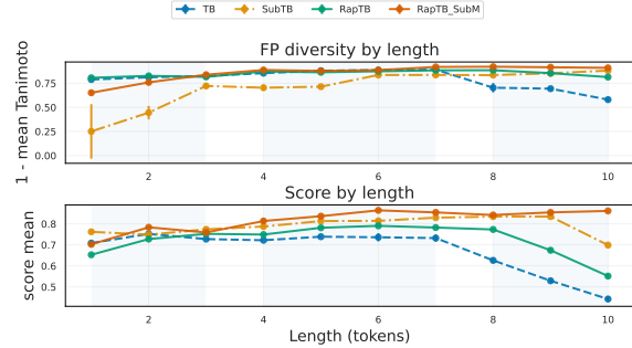
(b) Valid-only score and FPDiv versus length.
