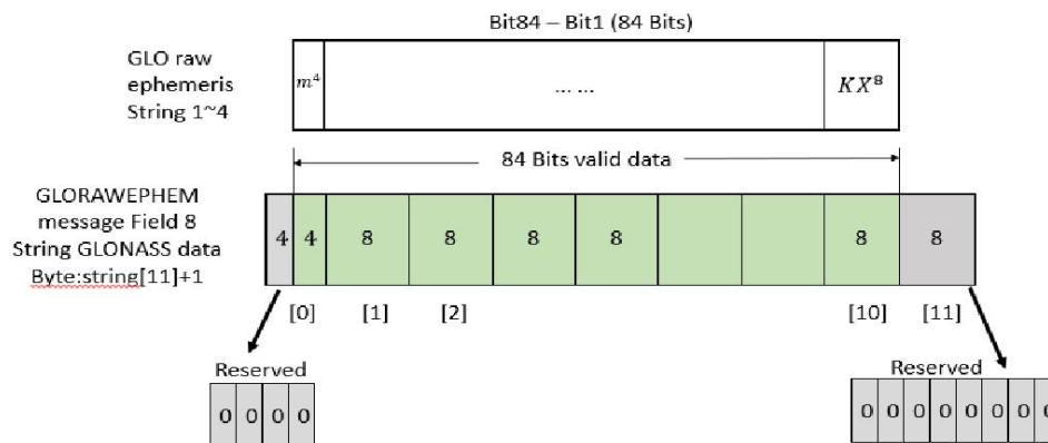
Fig 3-3 Structure of the GLONASS Raw Ephemeris Stream
