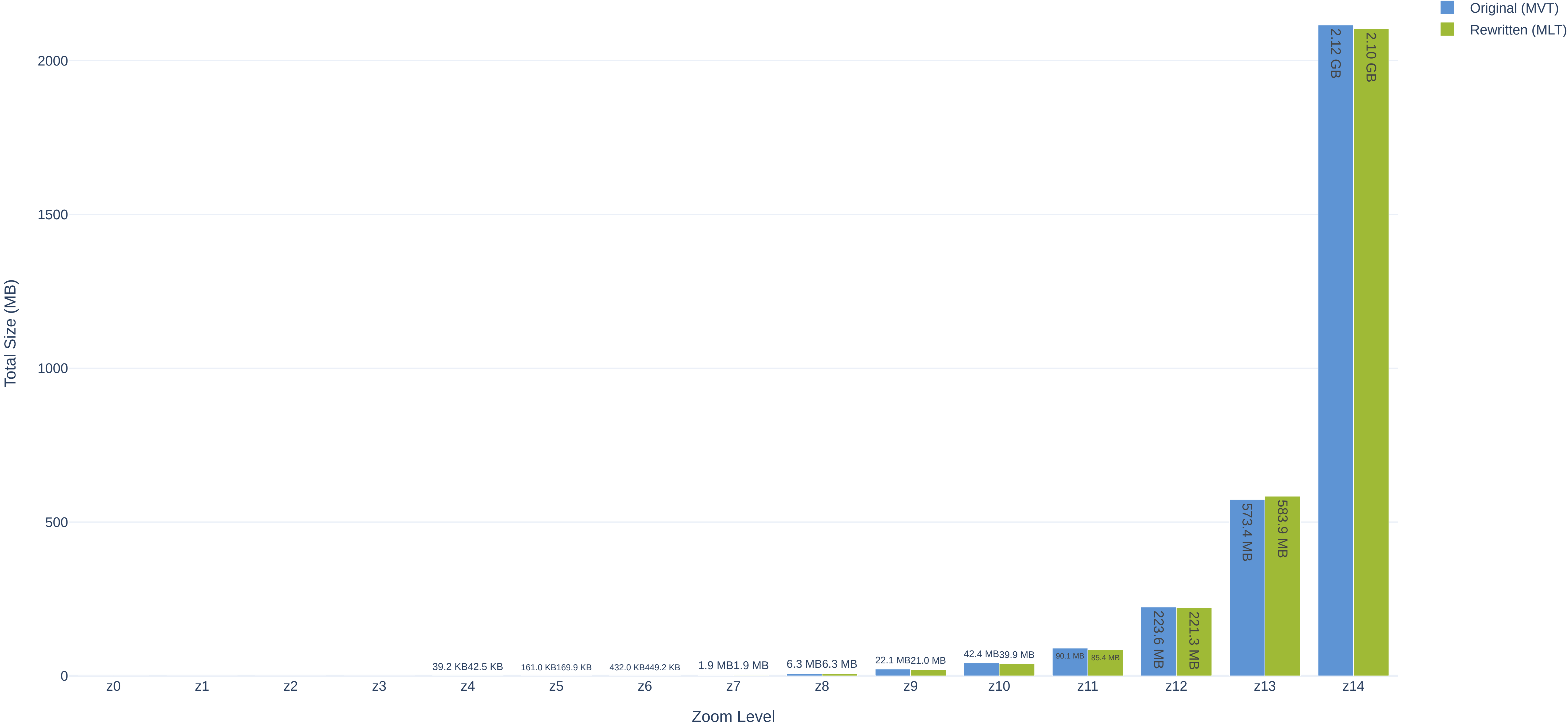
Total Tile Size per Zoom Level (overall: 3.08 GB → 3.06 GB, 0.4% reduction)
