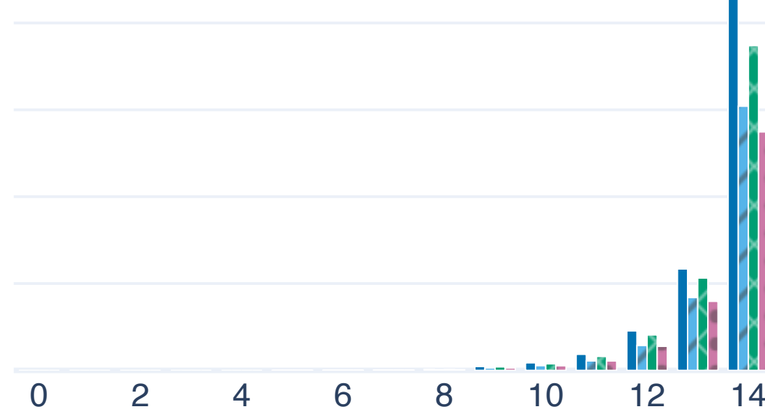
Zstd
