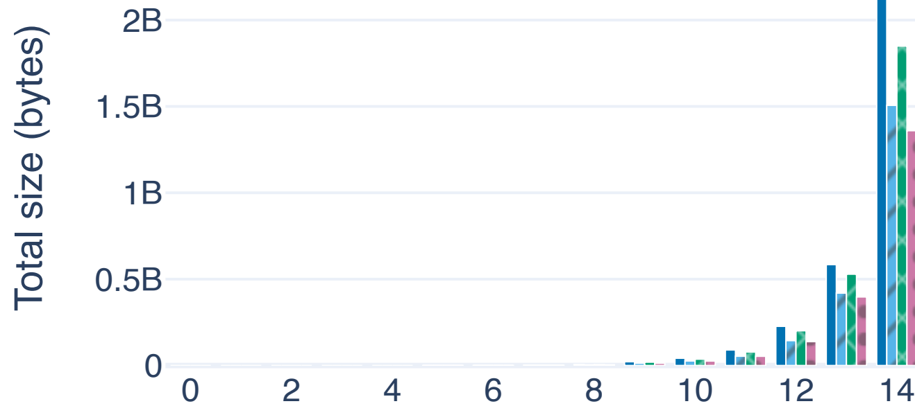
Brotli
