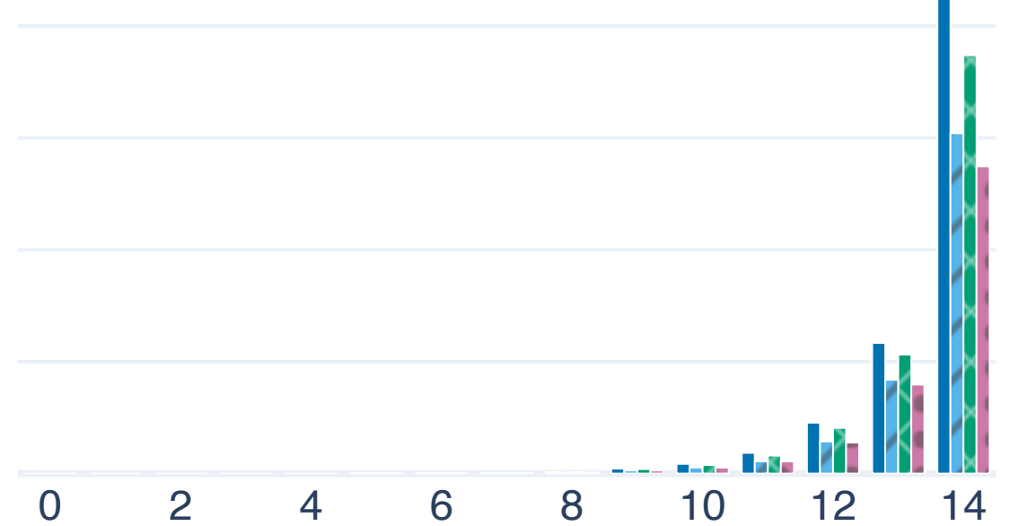
Zstd
