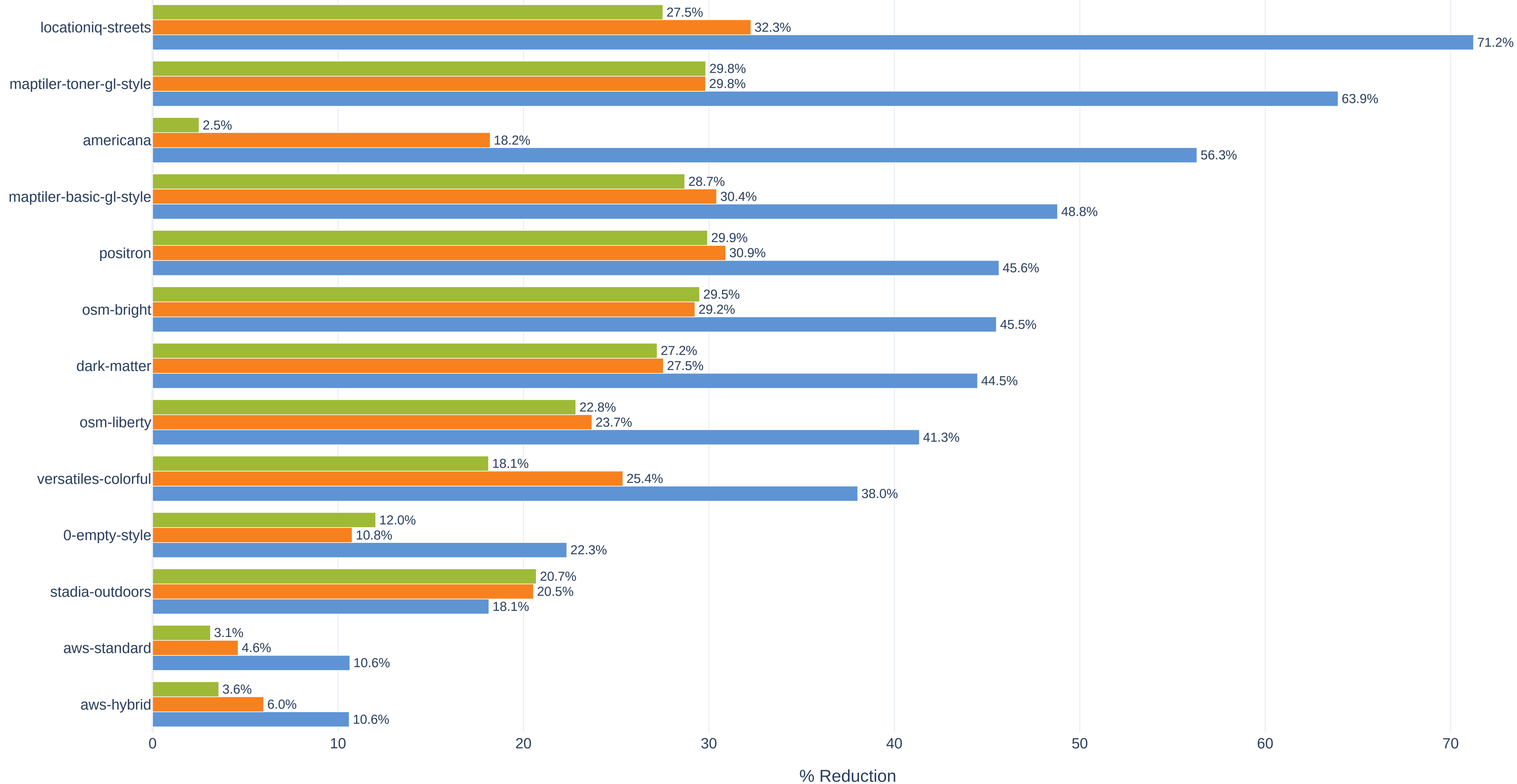
Size Reduction per Style (Raw, Gzip, Brotli)
