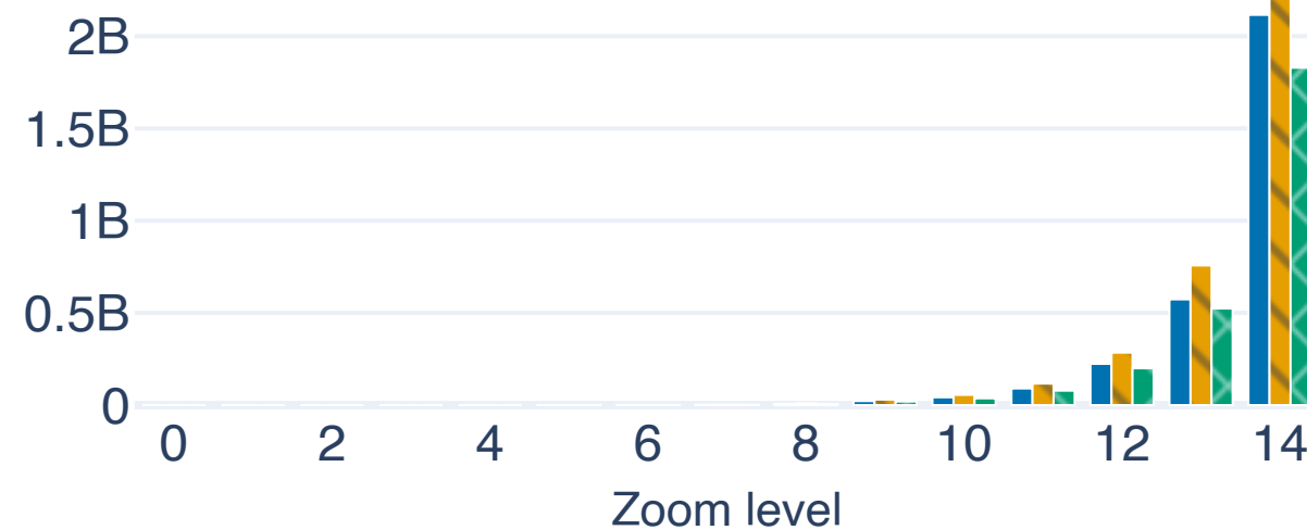
Zstd
