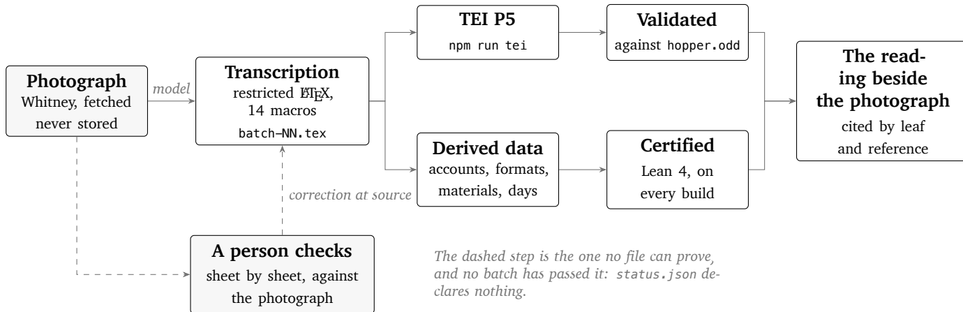
Figure 1: How a reading is made and what is derived from it. Every arrow but the dashed pair is a script that runs on each build and fails loudly; the dashed pair is the human check, which alone changes a batch’s state and which no file can vouch for. The sibling editions of Section 8 run the same pipeline with another corpus in the first box.
