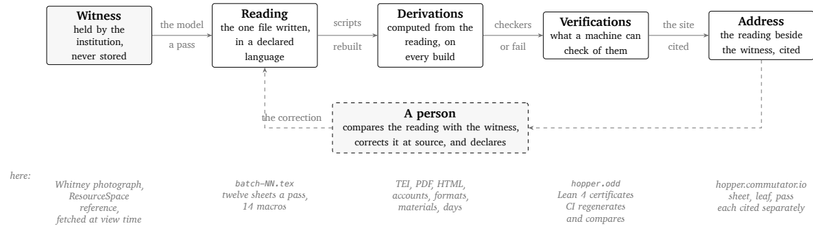
Figure 1: The schema the four editions of Section 8 share, and its values in this one. Five stations and one loop: the model turns a witness into a reading, in passes whose header names the model and the date; scripts derive everything else from the reading and regenerate it on every build; checkers fail the build on what a machine can check; the site places the reading beside the witness and cites both by reference. The dashed loop is the person, who compares the reading with the witness and corrects the reading, which alone changes anything downstream. Four invariants hold at every station: the witness is never stored; only the reading is written, everything else is derived and compared; every assertion carries an address into the witness; and the person’s verdict is declared, not observed. The grey row gives this edition’s values; the siblings’ are in Table 7.
