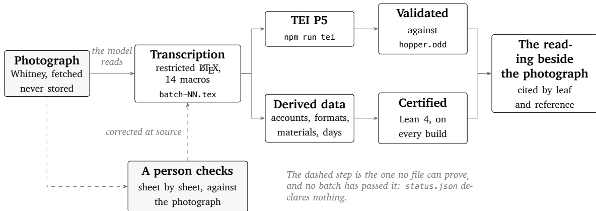
Figure 1: How a reading is made and what is derived from it. Every arrow but the dashed pair is a script that runs on each build and fails loudly; the dashed pair is the human check, which alone changes a batch’s state and which no file can vouch for. The sibling editions of Section 8 run the same pipeline with another corpus in the first box.
