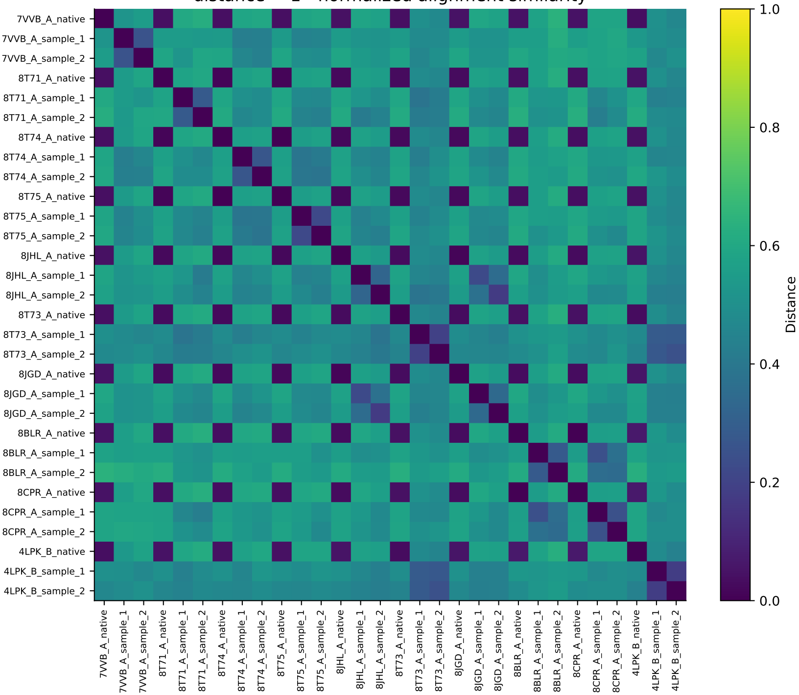
Pairwise distance heatmap from proteinmpnn_generated_sequences_reevaluated.fa distance = 1 - normalized alignment similarity
