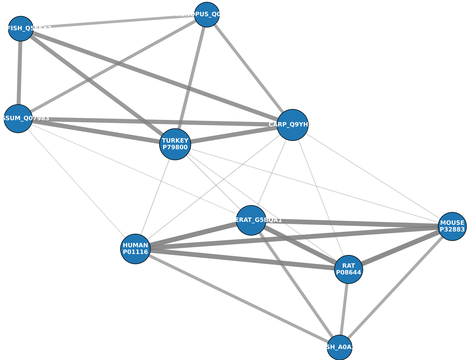
Sequence similarity network from kras_homologs_10.fasta Biopython PairwiseAligner + BLOSUM62, threshold = 0.88
