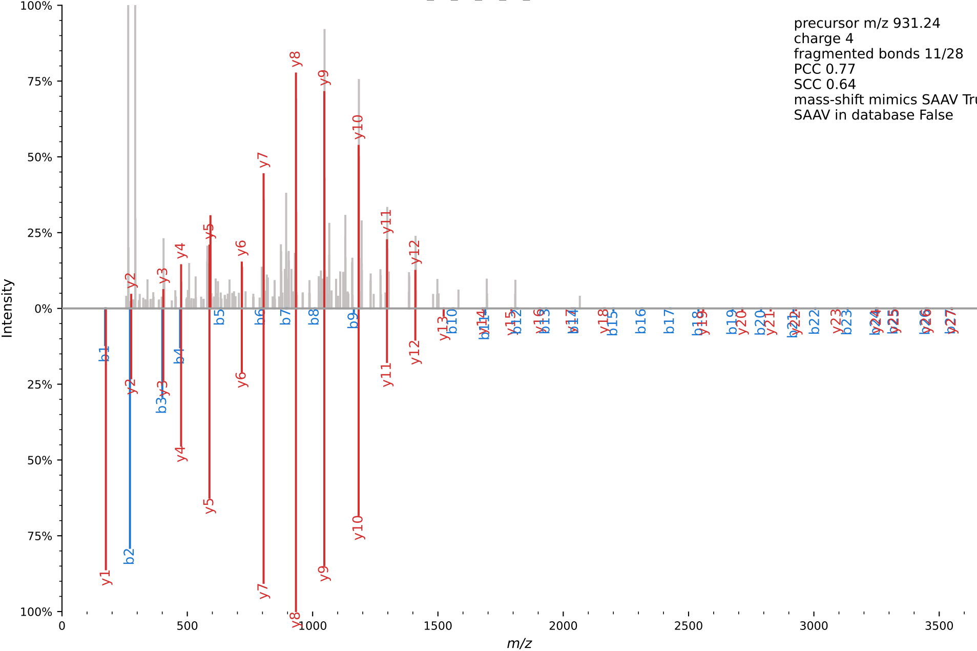
Annotated Spectrum for [+42.0106]-EVEAC[+57.0215]YTLRT[+294.0951]EQLNRILLHLESELAQTR file=130327_o2_06_hu_P3_2hr.mzXML scan=29345
