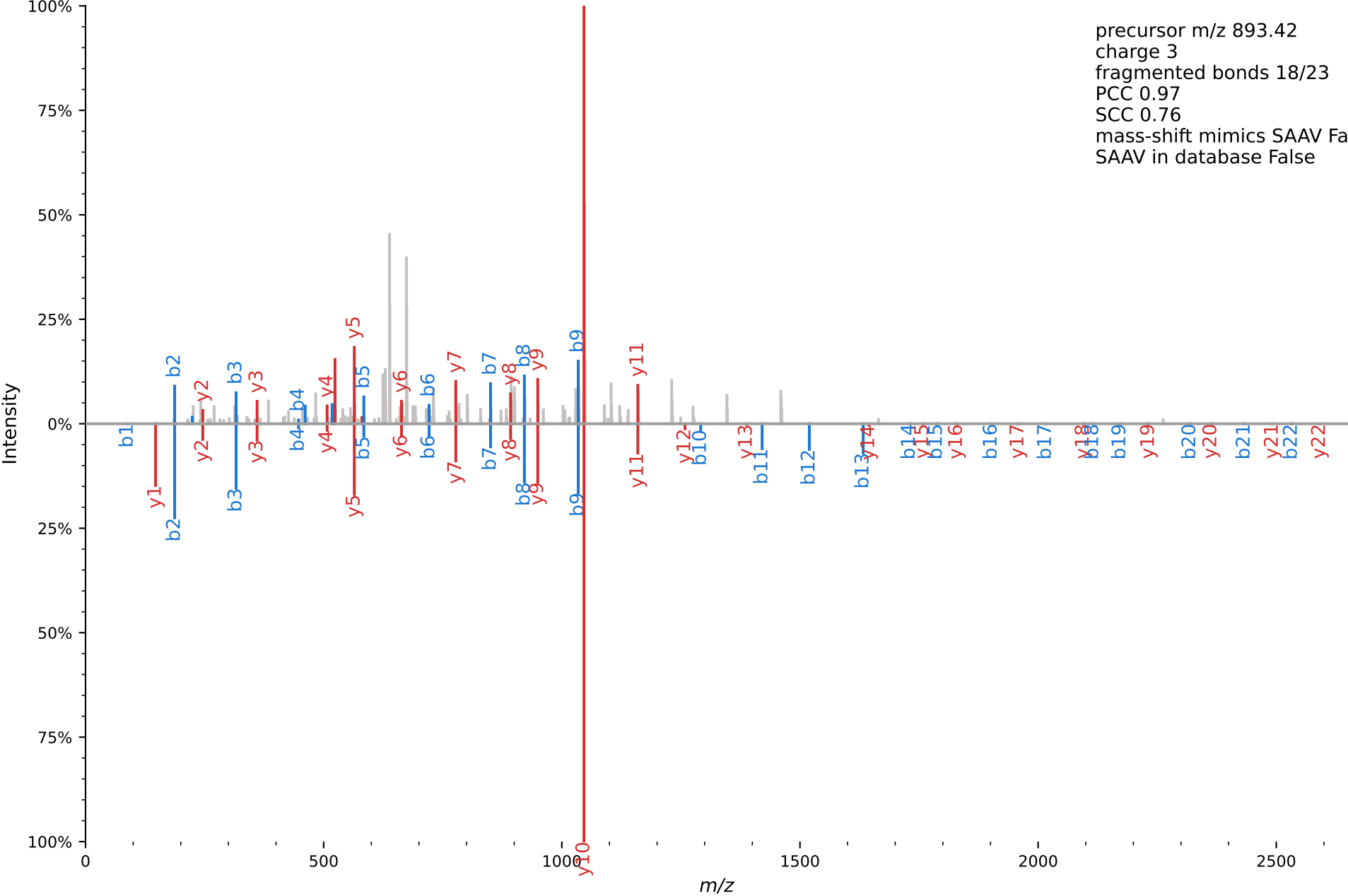
Annotated Spectrum for SVEMHHEALS[+170.0133]EVLPGDNVGFNVK file=AM14.mzXML scan=22752
