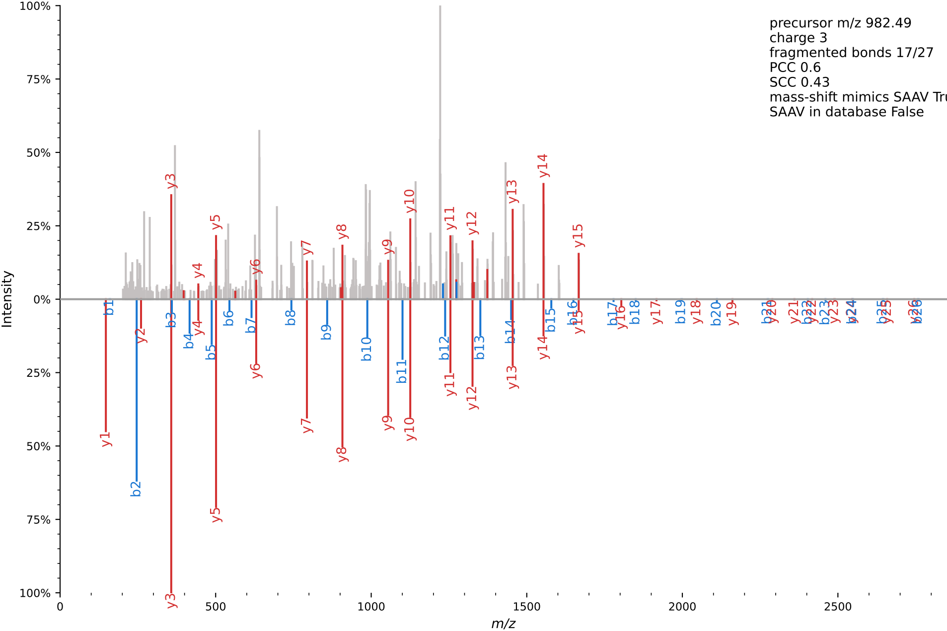
Annotated Spectrum for [+59.036279]-VSLGAGAKDELHIVEAEAM[+15.9949]NYEGSPIK file=AM16.mzXML scan=27588
