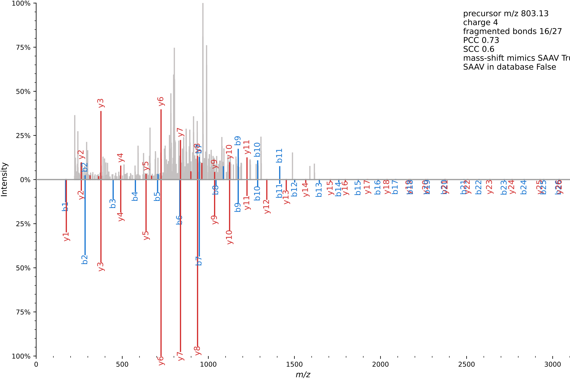
Annotated Spectrum for [+42.0106]-QLYEEEIPELQSQ[+14.9997]ILDTSVVLSM[+15.9949]DNSR file=AM9.mzXML scan=30462
