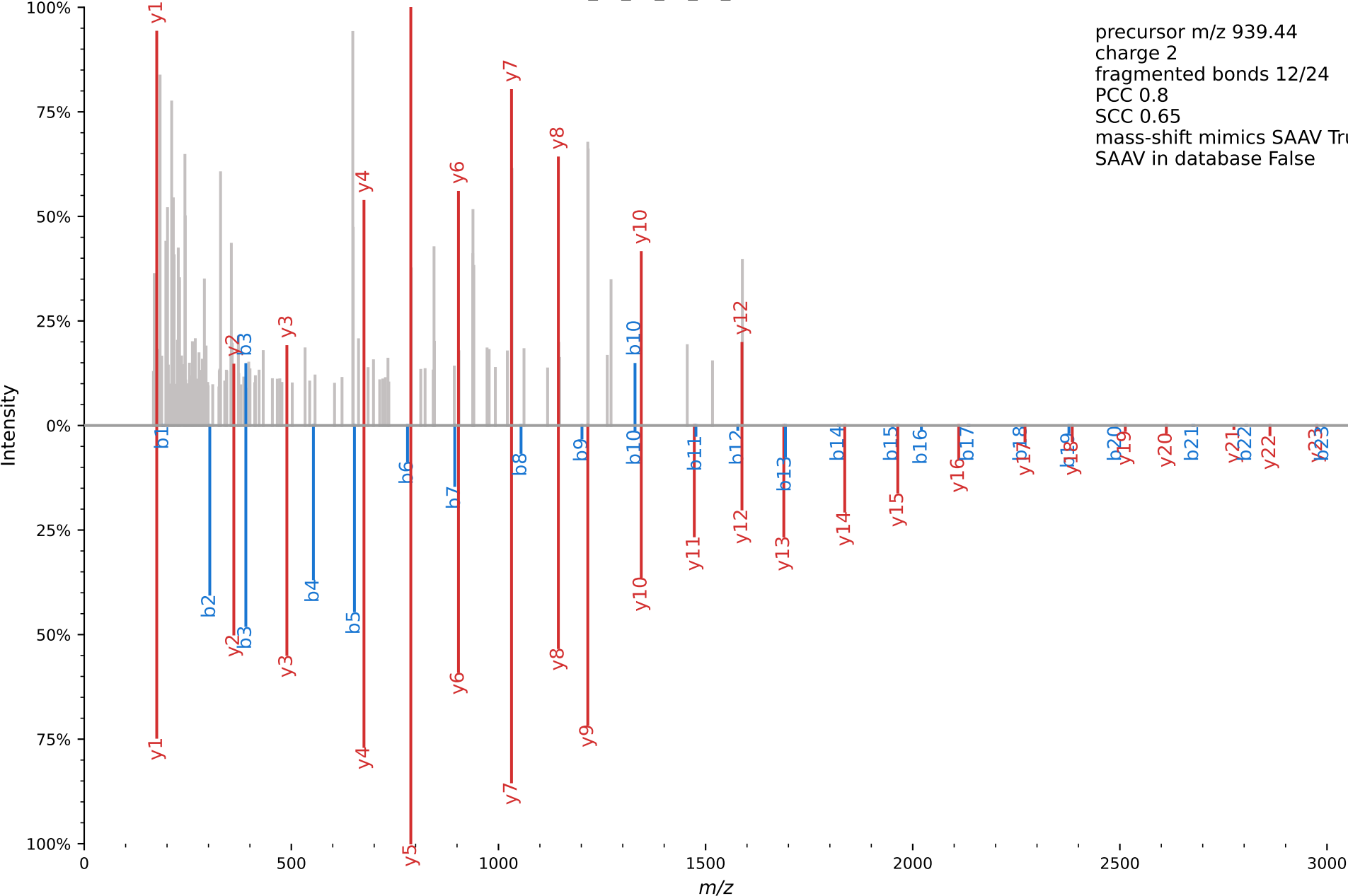
Annotated Spectrum for [+42.0106]-FISYVKNC[+57.0215]FQM[+15.9949]TDQEAIQLWQWR file=130327_o2_02_hu_P1_2hr.mzXML scan=31025
