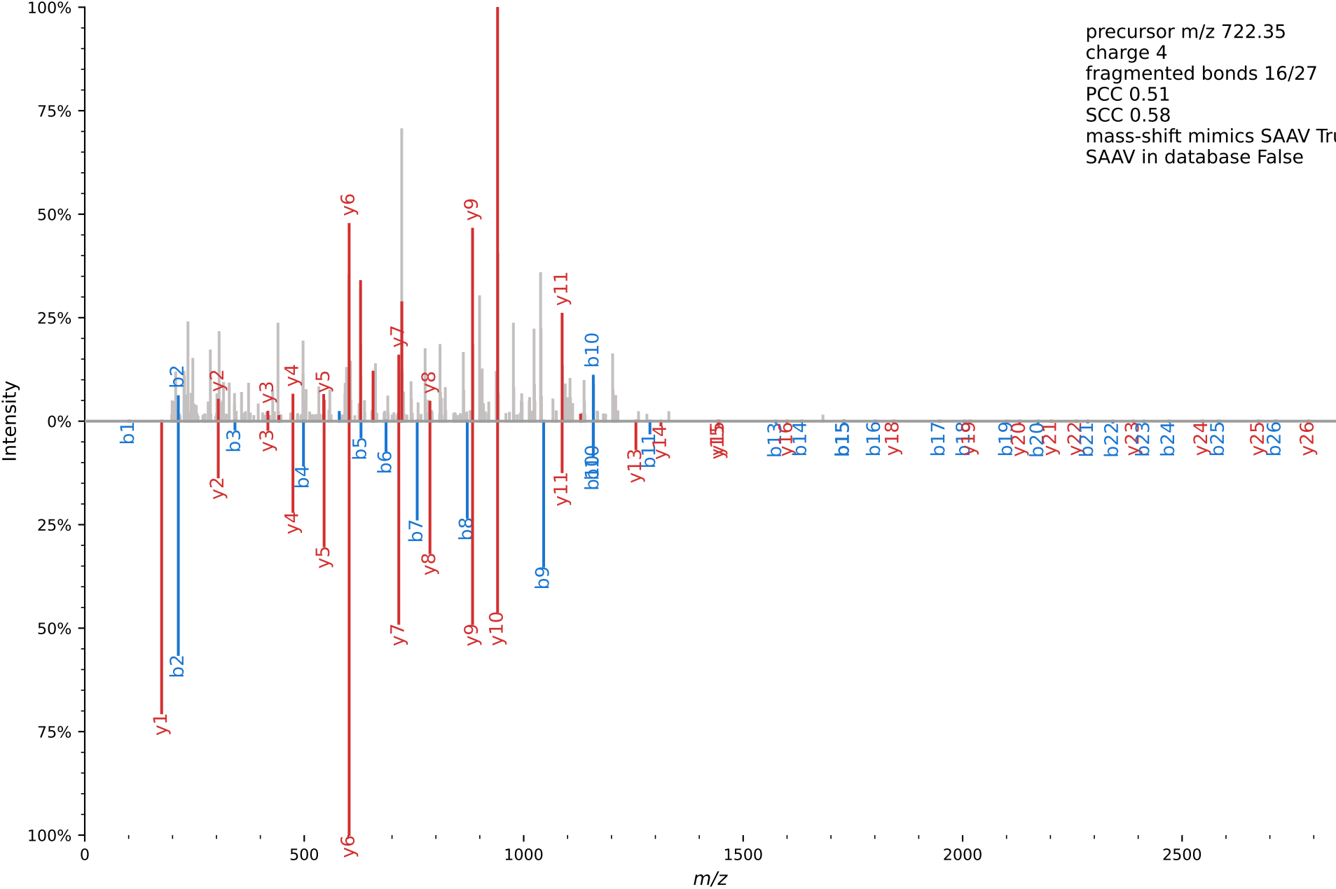
Annotated Spectrum for [+42.0106]-GLERMGANS[+87.0507]LERMGPMAM[+15.9949]GPALGAGIER file=AM11.mzXML scan=17154
