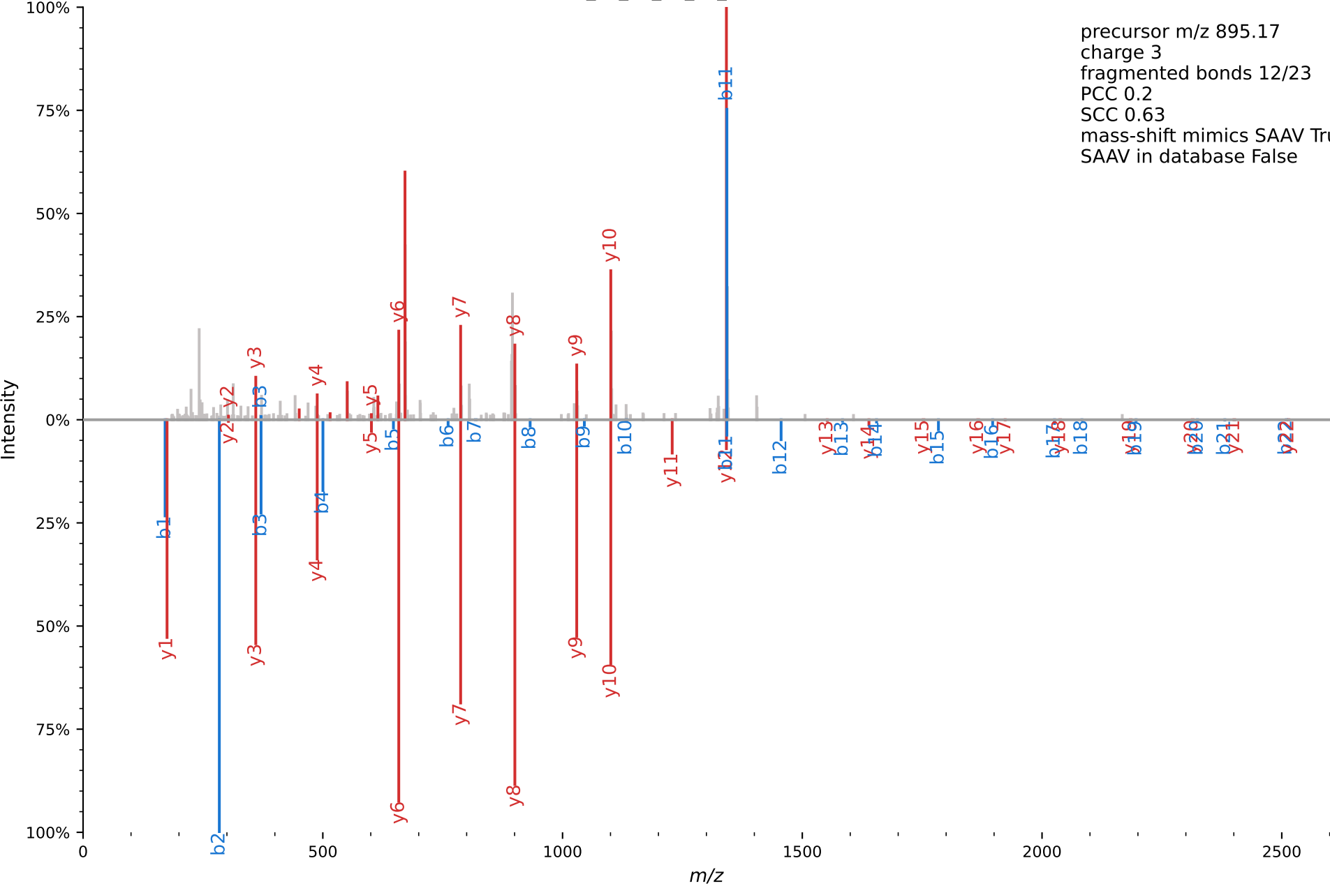
Annotated Spectrum for [+42.0106]-QISEM[+15.9949]NGNISR[+54.113505]LQAEIEGLKGQR file=130327_o2_06_hu_P3_2hr.mzXML scan=9557
