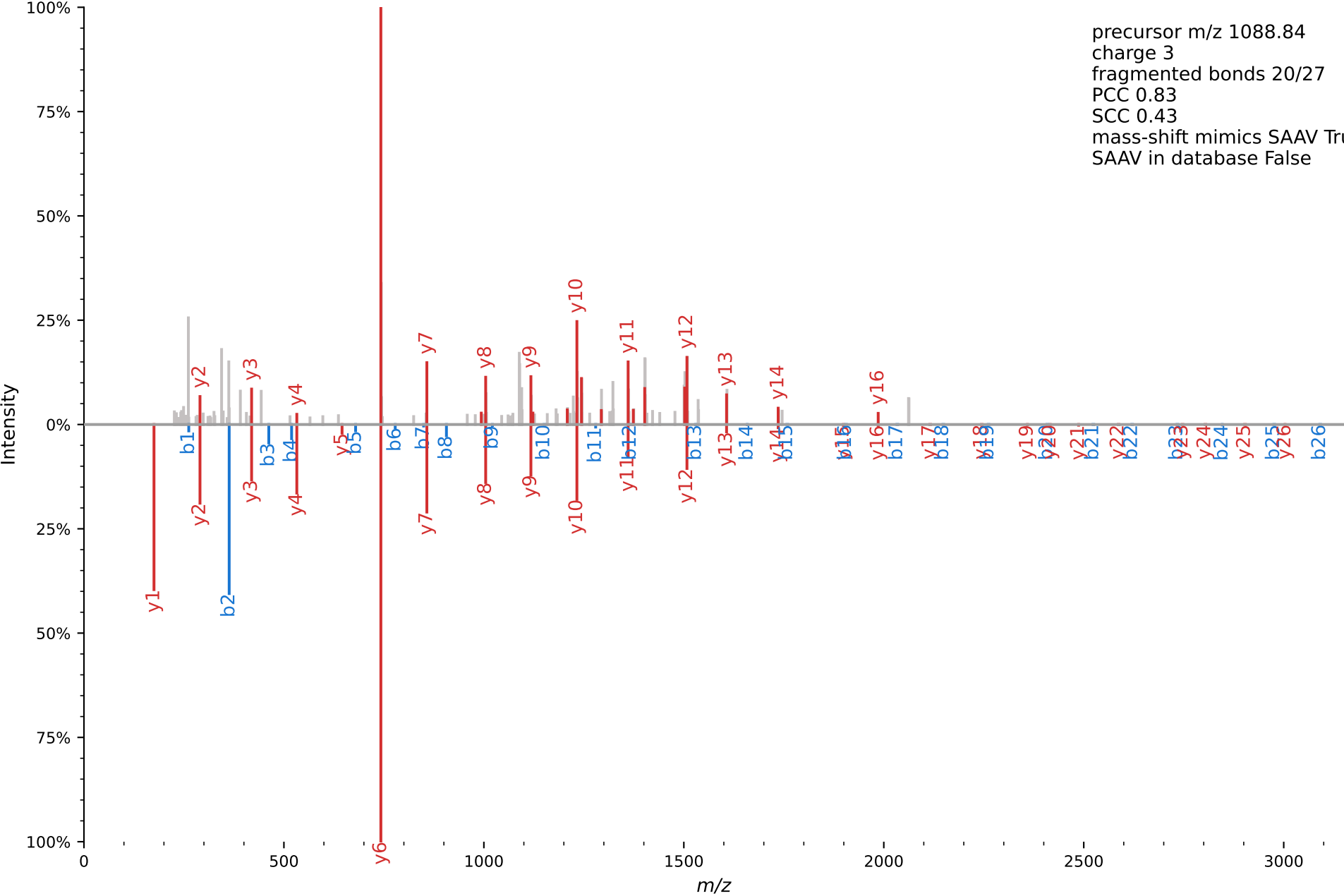
Annotated Spectrum for [+114.0429]-M[+15.9949]TVGC[+57.0215]VAGDEESYEVFKDLFDPIIEDR file=AM13.mzXML scan=32728
