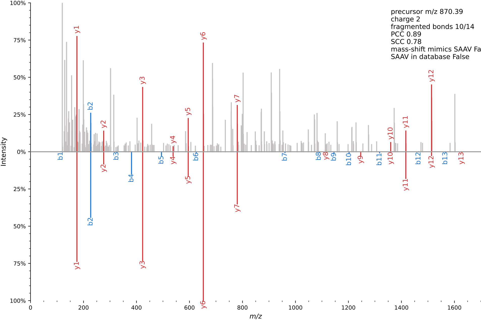
Annotated Spectrum for IIPGLMC[+232.0644]QGGDFTR file=AM16.mzXML scan=26469
