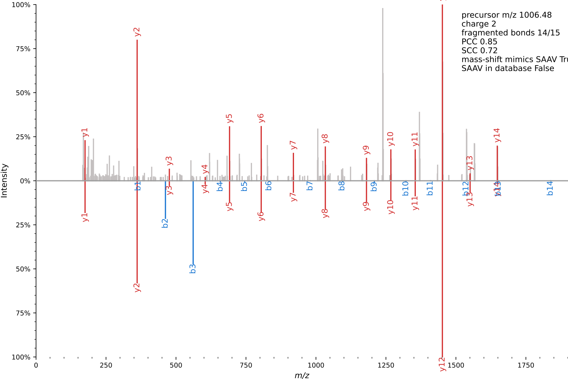
Annotated Spectrum for [+217.1688]-M[+15.9949]PVPSSFNDISQDWR file=AM16.mzXML scan=29960
