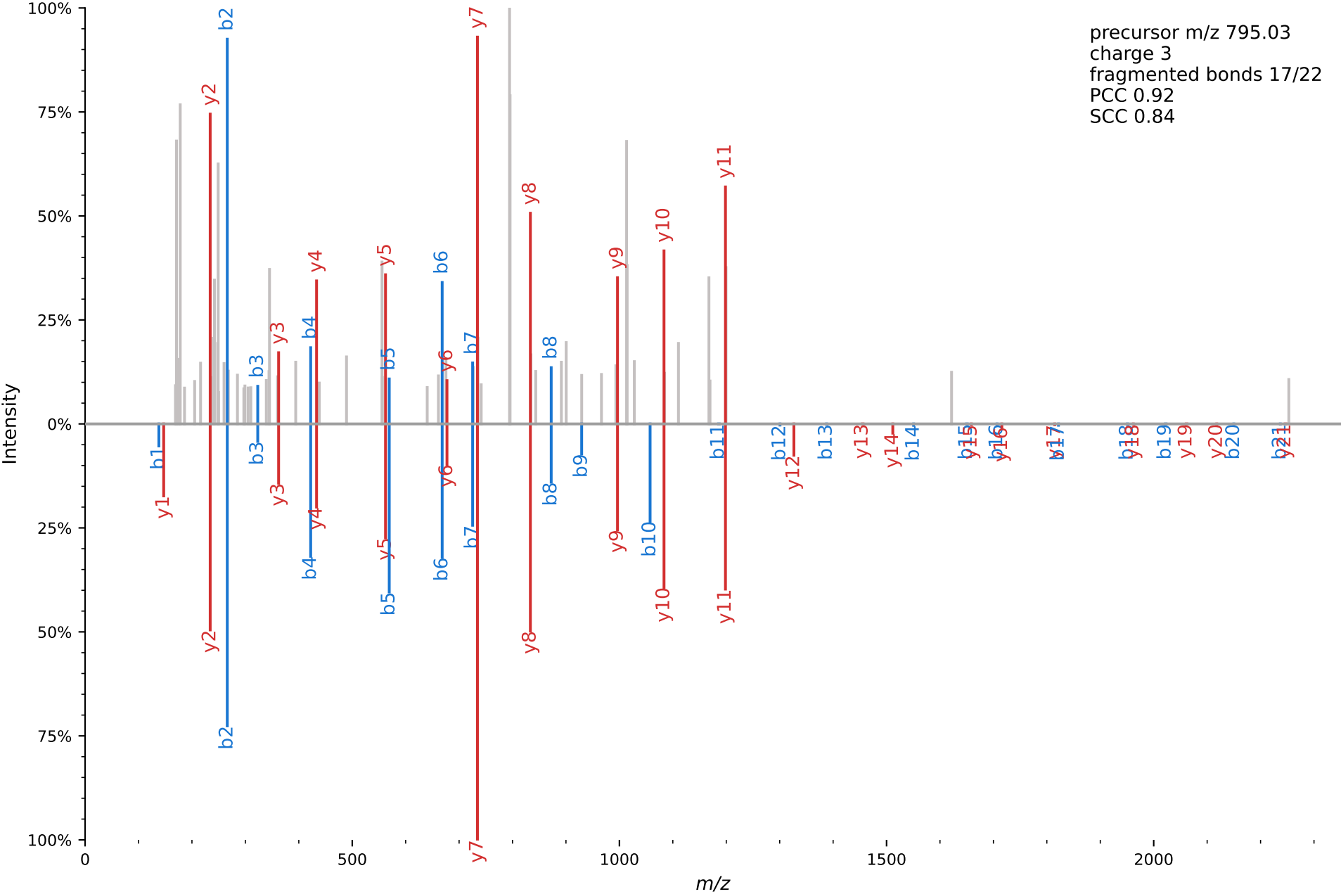
Annotated Spectrum for HQGVM[+15.9949]VGM[+15.9949]GQKDSYVGDDQ[+0.984]AQSK file=AM9.mzXML scan=10075
