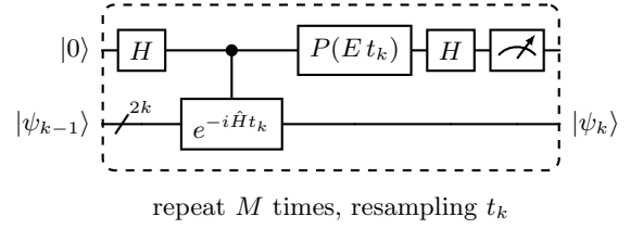
FIG. 10. One cycle of the rodeo algorithm: Hadamard on the ancilla, controlled time evolution e^{-i\hat{H}t_k} of the 2k -qubit system register with a Gaussian-random time t_k , ancilla phase P(Et_k) , second Hadamard, and a mid-circuit measurement of the ancilla, which is then reset and reused for the next cycle. A run is accepted when all M outcomes read 0; each accepted cycle applies the filter \frac{1}{2}(\mathbb{I} + e^{iEt_k}e^{-i\hat{H}t_k}) to the system. Unlike the VQE of Fig. 9(a), the circuit carries no variational parameters and no classical optimization loop; the controlled evolution, compiled from the same Pauli-rotation blocks as Fig. 9(b) with only the central R_z controlled, is the sole system-size-dependent element ( \approx 4.2 \times 10^2 CNOTs per Trotter step at k = 4 ).
