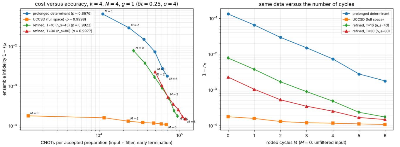
FIG. 12. Matched-observable comparison of inputs to the same Trotterized rodeo filter ( k = 4 , N = 4 , g = 1 ; second order, \delta t = 0.25 , \sigma = 4 , 40 common Gaussian time sets): the prolonged k = 2 determinant, the full-space gate-level UCCSD state, and the Trotterized resolution-refined state at T^* = 16 and T = 30 (the refinement cost includes the coarse term of Eq. (4)). Left: acceptance-weighted ensemble infidelity of the accepted runs versus CNOTs per accepted preparation, Eq. (10), as the number of cycles grows from M = 0 (unfiltered input; omitted for the gate-free determinant) to M = 6 . Right: the same infidelities versus M . All inputs converge to the floor set by the product formula; the UCCSD input reaches it first and cheapest.
