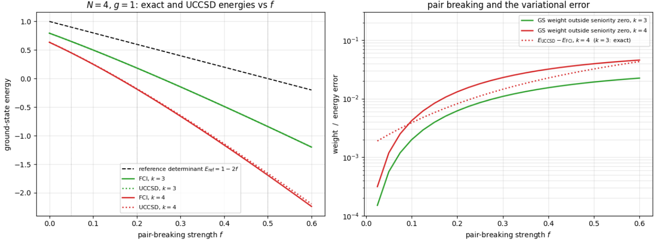
FIG. 13. The pairing model with the particle-hole term, N = 4 , g = 1 , as a function of the pair-breaking strength f . Left: energy of the reference determinant (dashed), exact ground-state energy (solid) and UCCSD energy (dotted) at k = 3 and k = 4 ; the vertical lines mark the strengths f = 0.05, 0.2, 0.5 of Table V. Right: weight of the exact ground state outside the seniority-zero subspace (solid) and the UCCSD energy error at k = 4 (dotted; at k = 3 the ansatz is exact).
