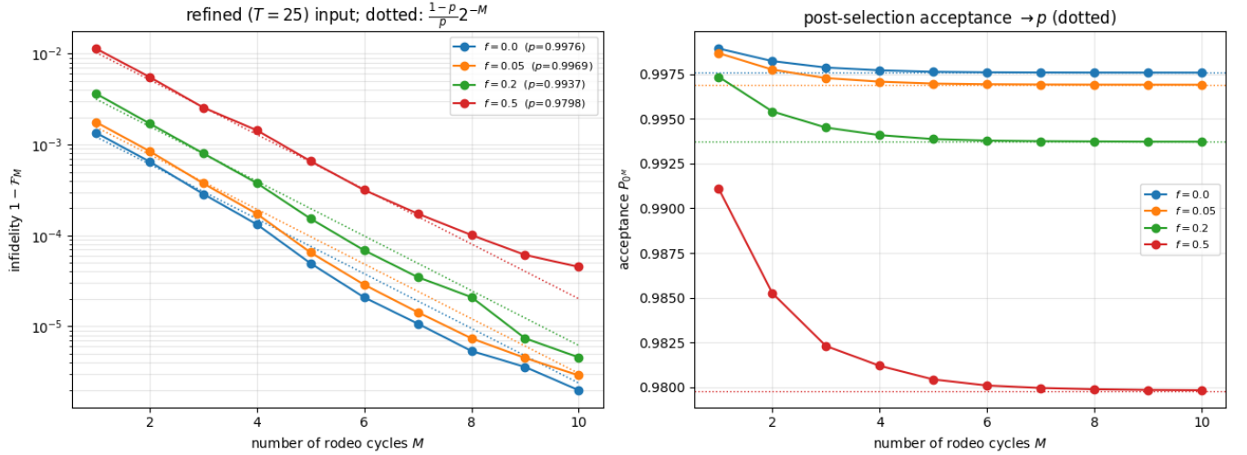
FIG. 16. Rodeo eigenstate preparation at E = E_0 with the particle-hole term, for f = 0, 0.05, 0.2, 0.5 , from the resolution-refined ( T = 25 ) input, averaged over 40 random time sets ( \sigma = 3 ). Left: post-selected infidelity versus the number of cycles M (dotted: \frac{1-p}{p}2^{-M} ). Right: the acceptance converges to the input overlap p (dotted).
