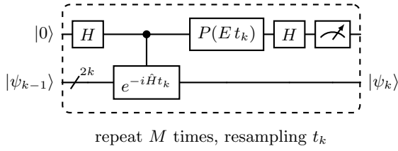
FIG. 10. One cycle of the rodeo algorithm: Hadamard on the ancilla, controlled time evolution e^{-iHt_k} of the 2k -qubit system register with a Gaussian-random time t_k , ancilla phase P(Et_k) , second Hadamard, and a mid-circuit measurement of the ancilla, which is then reset and reused for the next cycle. A run is accepted when all M outcomes read 0; each accepted cycle applies the filter \frac{1}{2}(\mathbb{I} + e^{iEt_k}e^{-iHt_k}) to the system. Unlike the VQE of Fig. 9(a), the circuit carries no variational parameters and no classical optimization loop; the controlled evolution, compiled from the same Pauli-rotation blocks as Fig. 9(b) with only the central R_z controlled, is the sole system-size-dependent element ( \approx 4.2 \times 10^2 CNOTs per Trotter step at k = 4 ).
