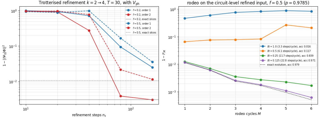
FIG. 17. The pipeline at the circuit level with the particle-hole term ( k = 4 , N = 4 , g = 1 ). Left: infidelity of the Trotterized refinement k = 2 \rightarrow 4 ( T = 30 ) versus the number of product-formula steps n_s for first- and second-order formulas at f = 0.2 (solid) and f = 0.5 (dashed); horizontal lines mark the exact-slice refinement. Right: rodeo infidelity versus cycles at f = 0.5 on the circuit-level refined input ( n_s = 80 , second order, p = 0.9785 ) with the controlled evolution Trotterized at fixed step sizes \delta t ; the legend gives the mean number of steps per cycle and the six-cycle acceptance.
