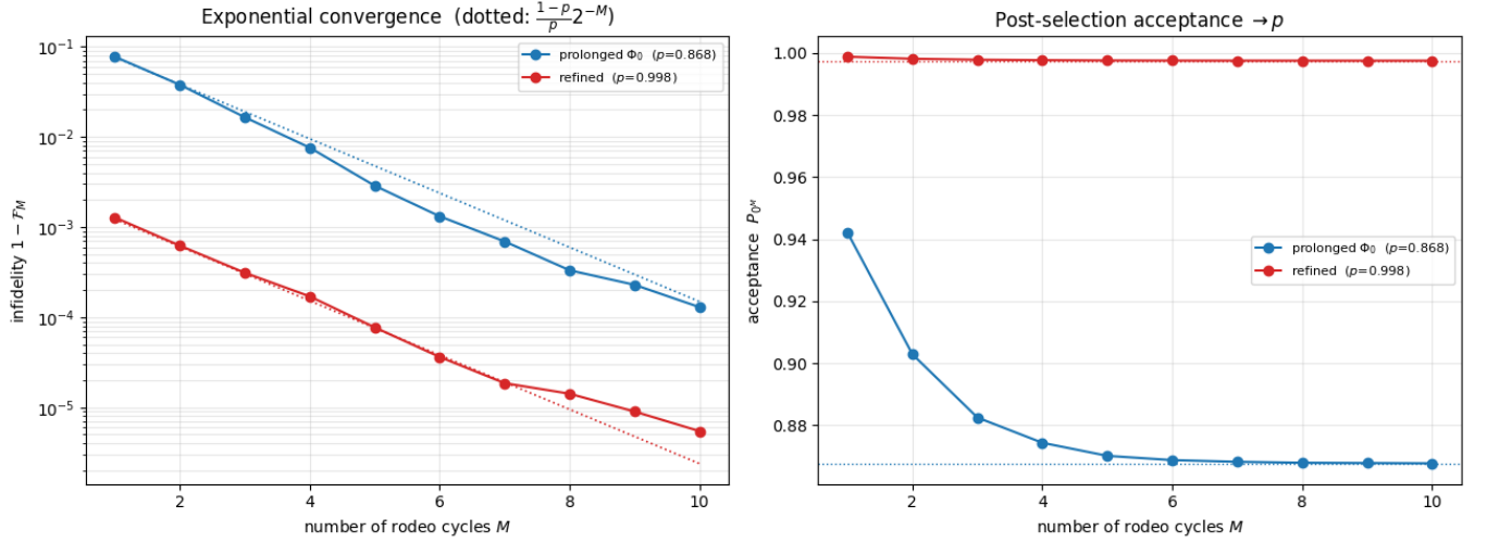
FIG. 8. Rodeo eigenstate preparation at E = E_0 ( k = 4 , N = 4 , g = 1 , \sigma = 3 ), averaged over 40 Gaussian time sets, for the resolution-refined input ( T = 25 , exact slices, p = 0.9976 ) and the prolonged determinant ( p = 0.868 ), with exact controlled evolution. Left: unweighted mean of the post-selected infidelity versus the number of cycles M (dotted: the analytic ensemble expectation of Eq. (8), which for these spectra coincides with \frac{1-p}{p}2^{-M} ). Right: the post-selection acceptance converges to the input overlap p .
