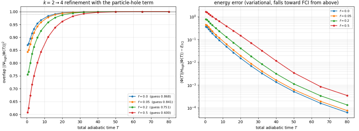
FIG. 14. Resolution refinement k = 2 \rightarrow 4 at N = 4 , g = 1 , for the pair-breaking strengths f = 0, 0.05, 0.2, 0.5 . Left: overlap with the exact ground state versus the adiabatic time T (legend: initial overlap of the prolonged determinant; dotted line: the 0.99 target). Right: variational energy error \langle \Phi(T) | H_{\text{high}} | \Phi(T) \rangle - E_{\text{FCI}} on a logarithmic scale.
