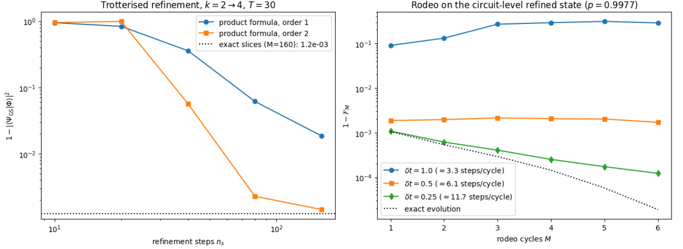
FIG. 11. The pipeline at the circuit level ( k = 4 , N = 4 , g = 1 ). Left: infidelity of the Trotterized refinement versus the number of product-formula steps n_s along the T = 30 path, for first- and second-order formulas; the dotted line is the exact-slice reference. Right: rodeo infidelity versus the number of cycles M for a Trotterized controlled evolution with fixed step size \delta t (input: the n_s = 80 circuit-level refined state, p = 0.9977 ). Too-coarse steps are rejected by the filter itself (the \delta t = 1 acceptance collapses to 0.10); \delta t = 0.25 tracks the exact evolution.
