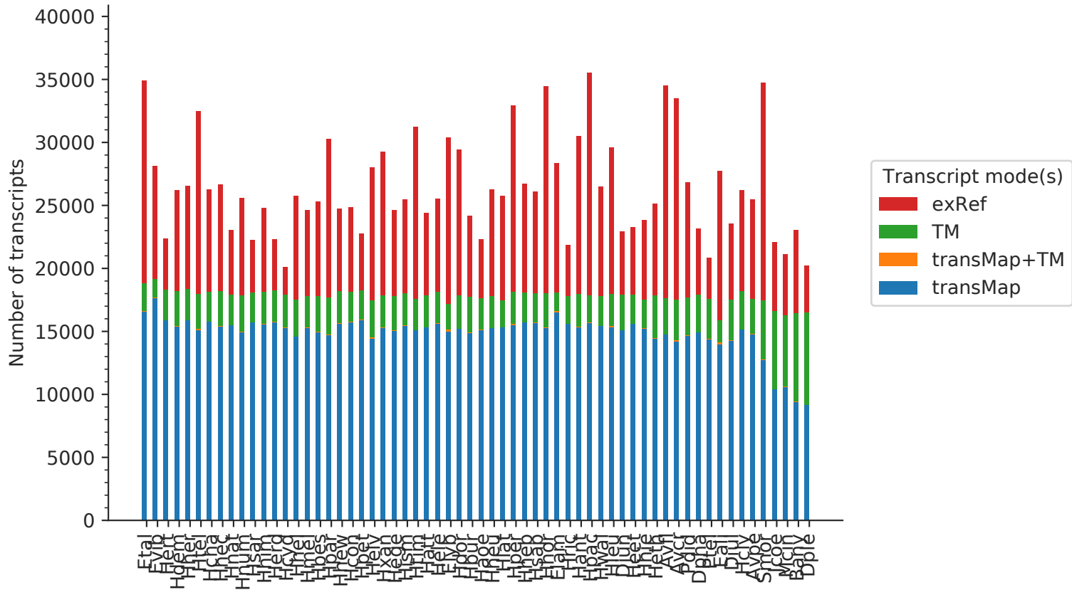
Transcript modes in protein coding consensus gene set
