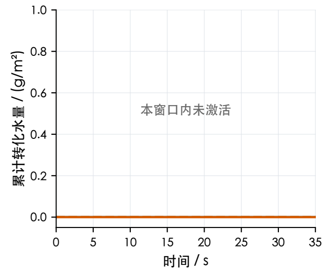
(c) 凝华
