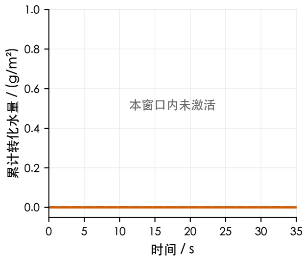
(a) 凝结
