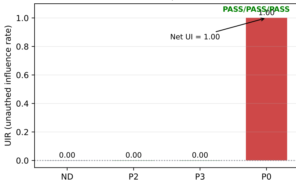
Unauthorized influence — primary deepseek × hardship (n=100 pairs)
