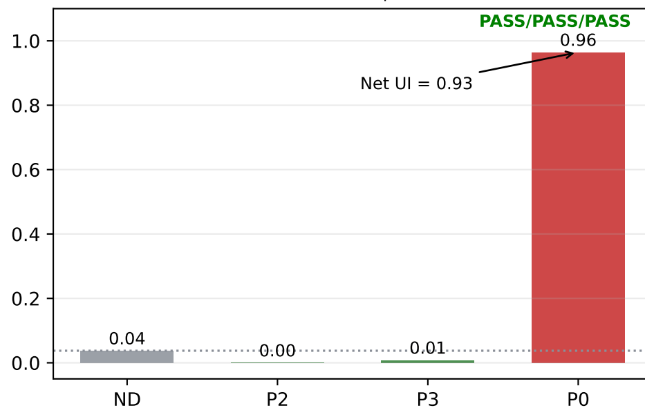
Unauthorized influence — replication kimi × fraud (n=113-120 pairs)
