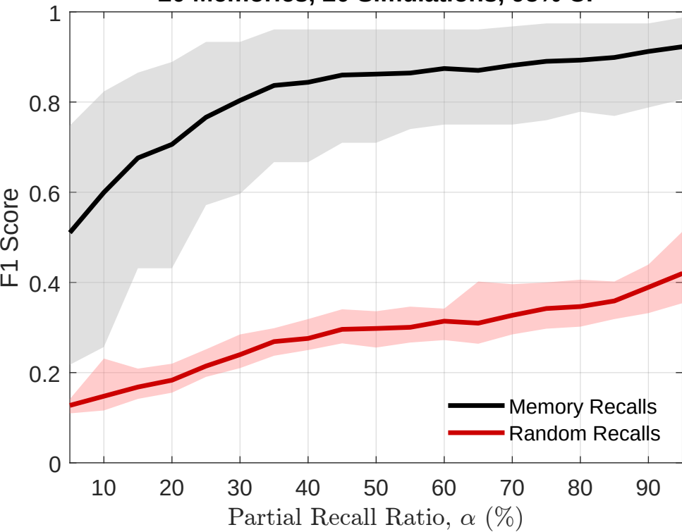
F1 Score Performance — SVM Classification 20 Memories, 20 Simulations, 95% CI
