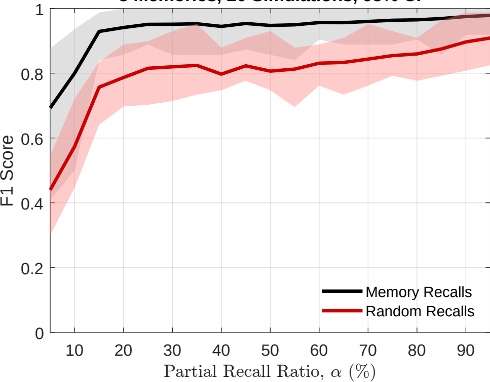
F1 Score Performance — SVM Classification 5 Memories, 20 Simulations, 95% CI
