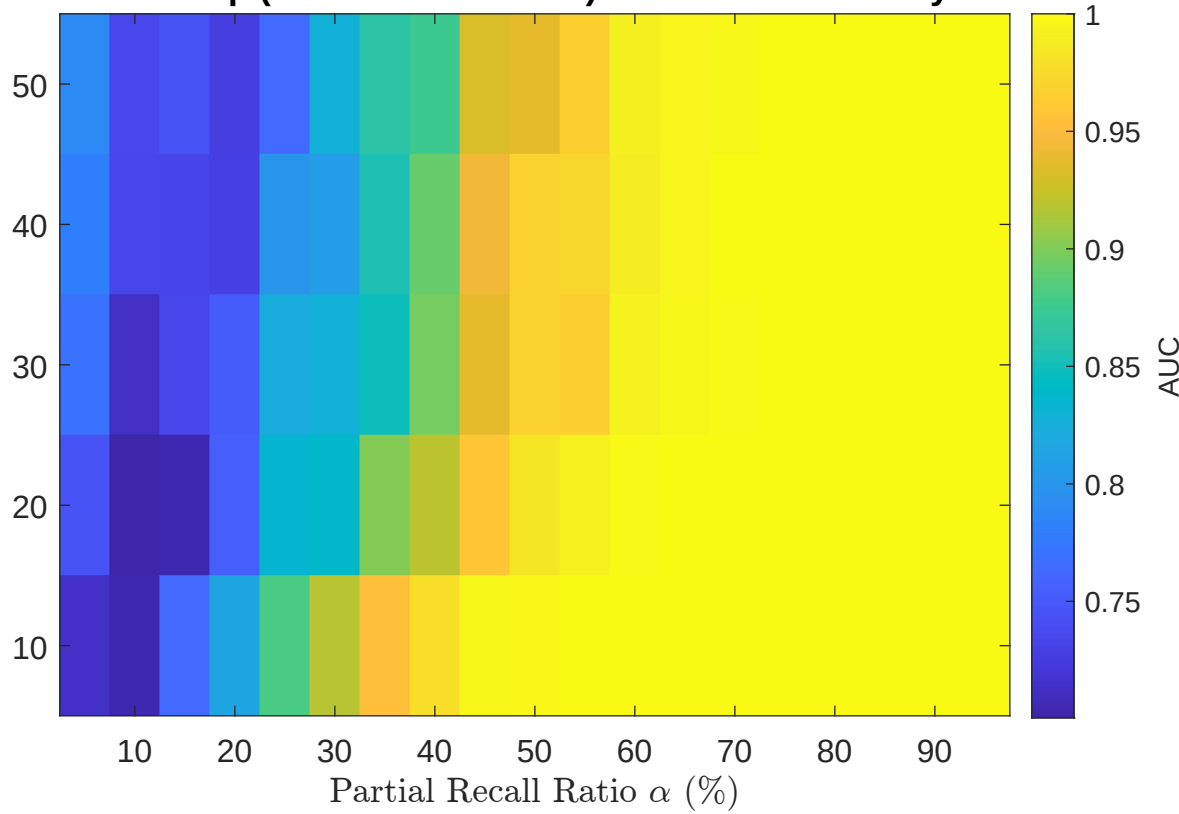
AUC Heatmap (SVM Classification) for Random Memory Class
