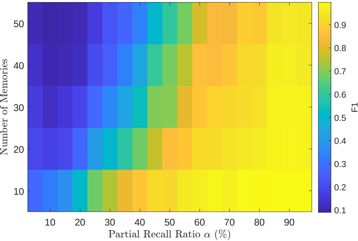
F1 Heatmap (SVM Classification) for Random Memory Class
