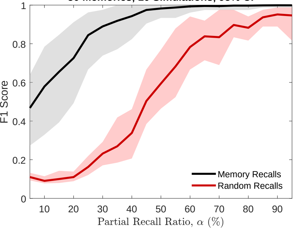
F1 Score Performance — SVM Classification 50 Memories, 10 Simulations, 95% CI
