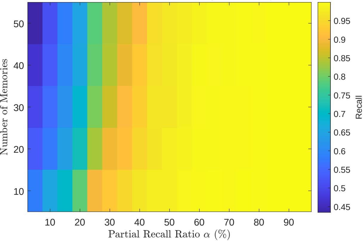
Recall Heatmap (SVM Classification) for Memory Class
