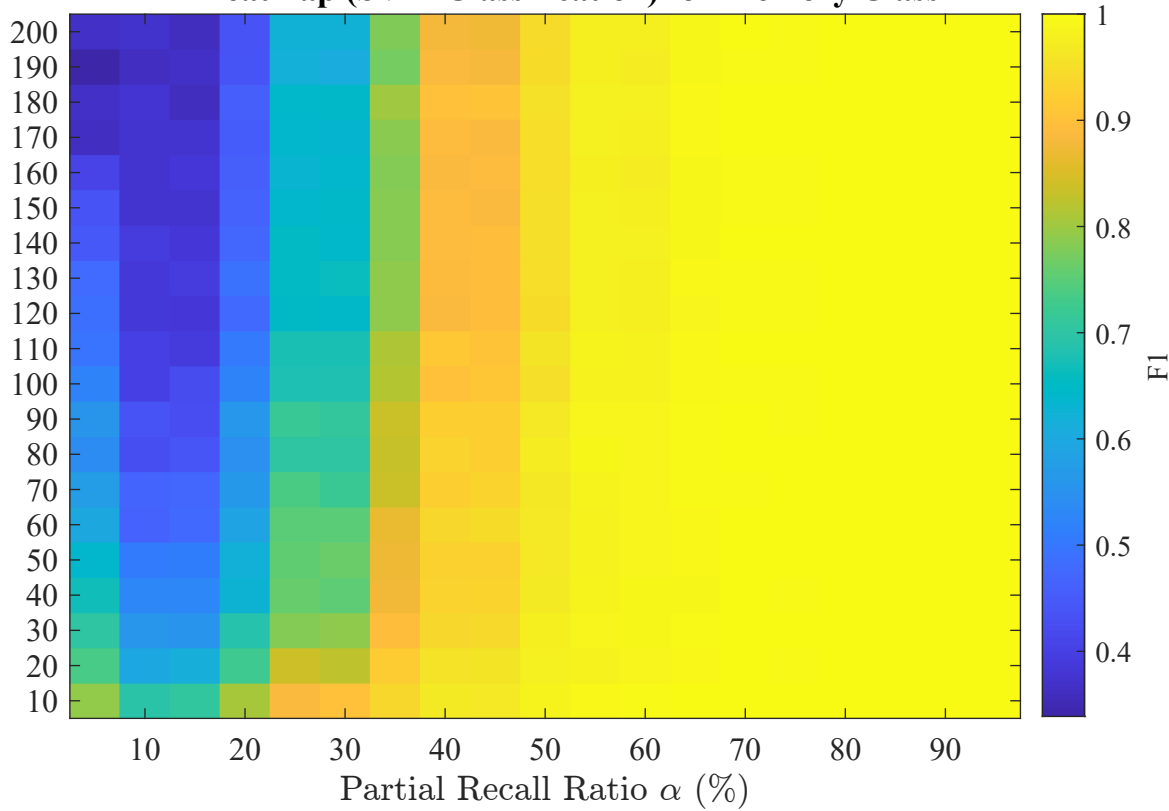
F1 Heatmap (SVM Classification) for Memory Class
