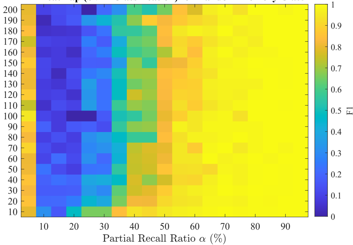
F1 Heatmap (SVM Classification) for Random Memory Class
