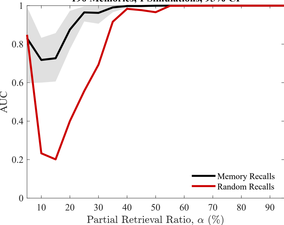
AUC Performance — SVM Classification 190 Memories, 1 Simulations, 95% CI
