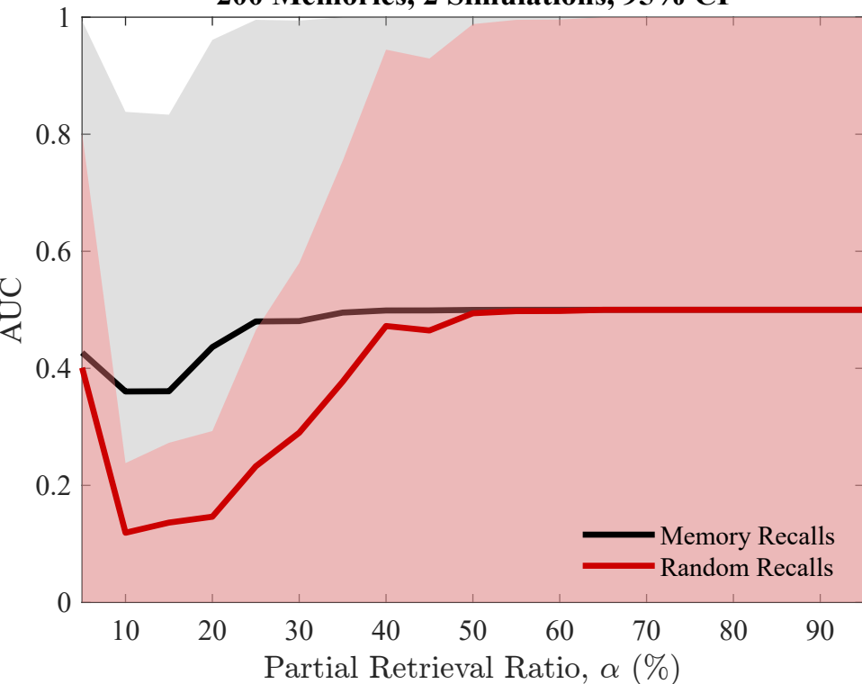
AUC Performance — SVM Classification 200 Memories, 2 Simulations, 95% CI
