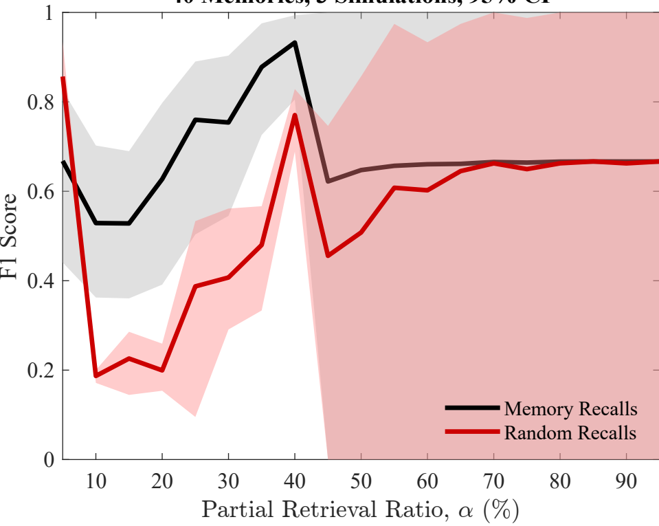
F1 Score Performance — SVM Classification 40 Memories, 3 Simulations, 95% CI
