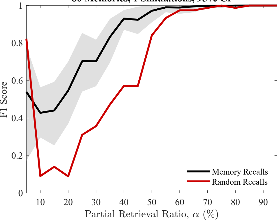
F1 Score Performance — SVM Classification 80 Memories, 1 Simulations, 95% CI
