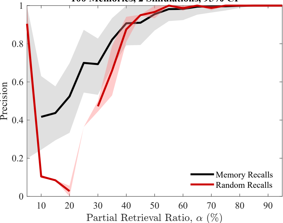
Precision Performance — SVM Classification 100 Memories, 2 Simulations, 95% CI
