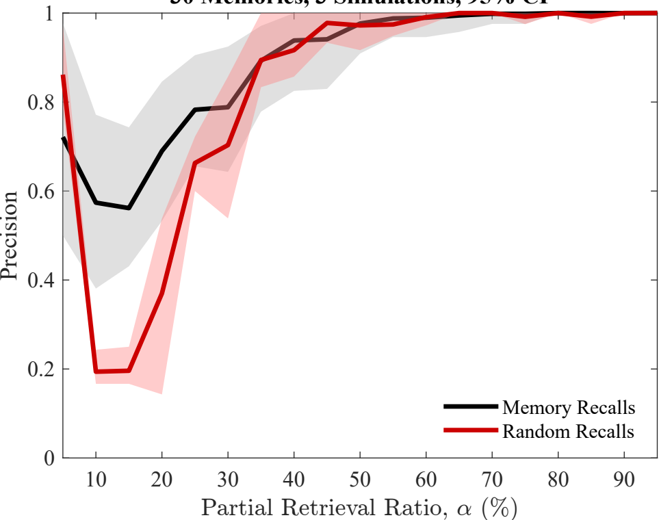
Precision Performance — SVM Classification 30 Memories, 3 Simulations, 95% CI
