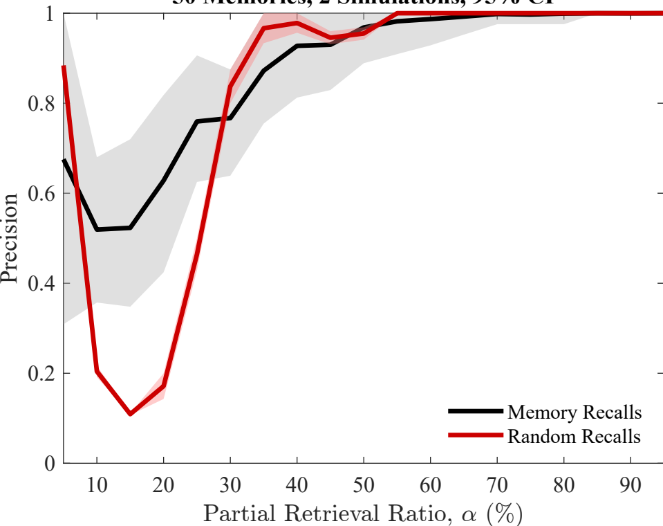
Precision Performance — SVM Classification 50 Memories, 2 Simulations, 95% CI
