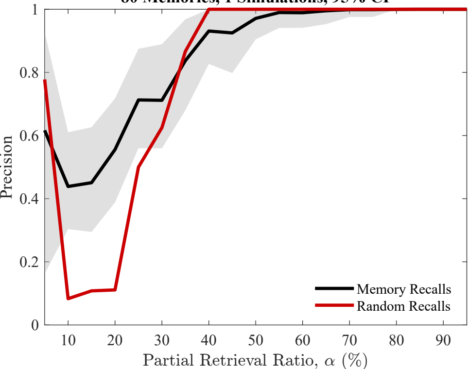
Precision Performance — SVM Classification 80 Memories, 1 Simulations, 95% CI
