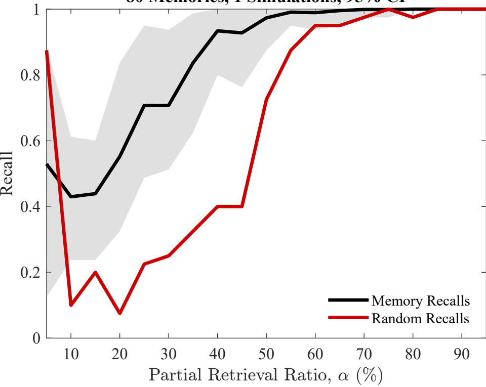
Recall Performance — SVM Classification 80 Memories, 1 Simulations, 95% CI
