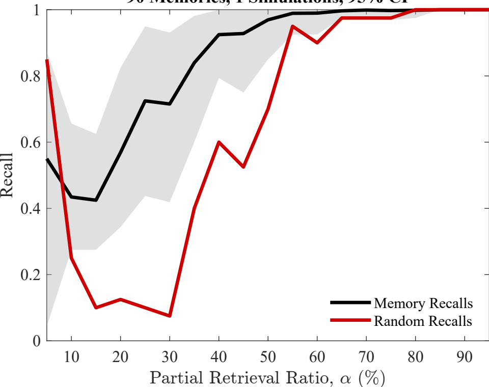
Recall Performance — SVM Classification 90 Memories, 1 Simulations, 95% CI
