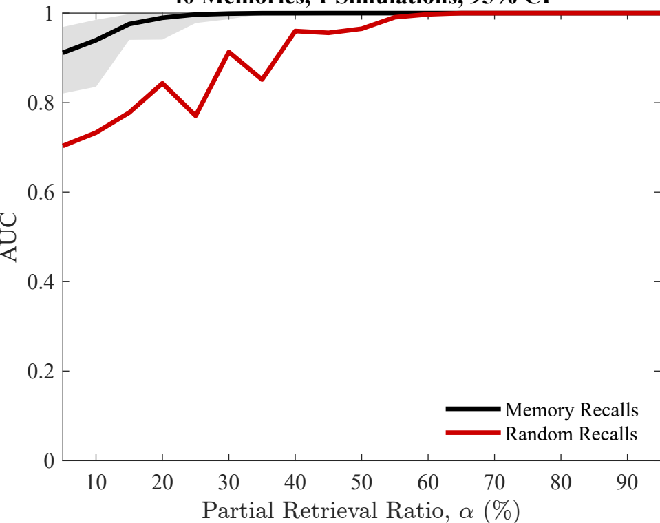
AUC Performance — SVM Classification 40 Memories, 1 Simulations, 95% CI
